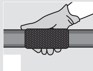
Rub and polish thoroughly. KEEP HANDS MOVING QUICKLY. WET GLOVES FREQUENTLY TO AVOID STICKING. Finished application.
