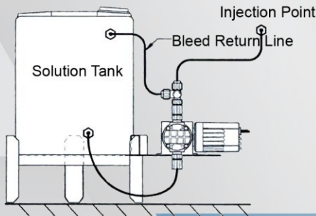
Typical Tank, Stand, Feeder Combination
