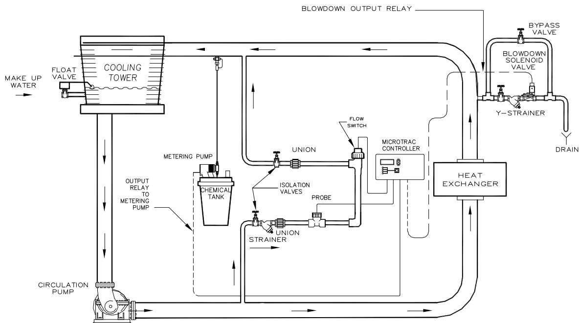
Fig. 1: Typical Installation
