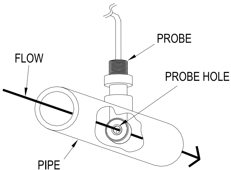
Fig. 1: Typical Installation
