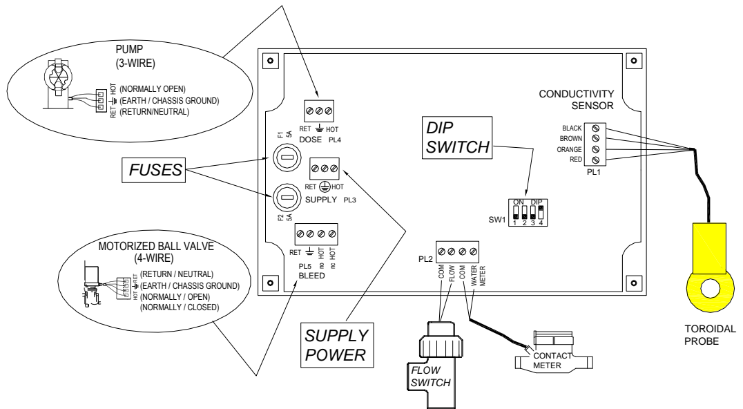
Fig. 3: Wire Connections 3
